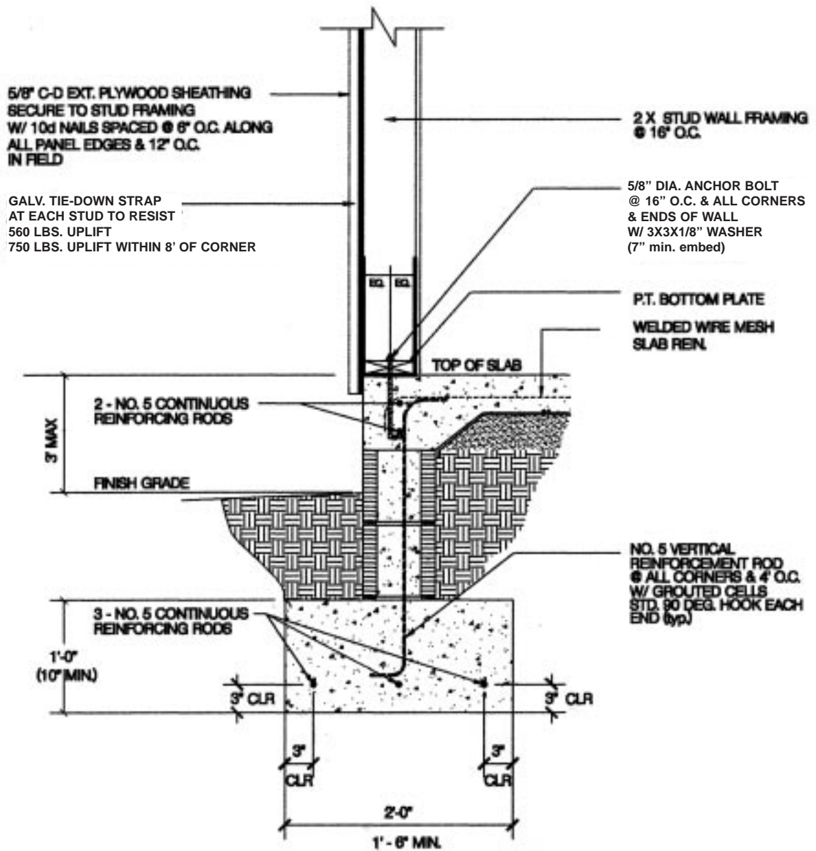
3 CMU STEM WALL W/ WOOD FRAME
