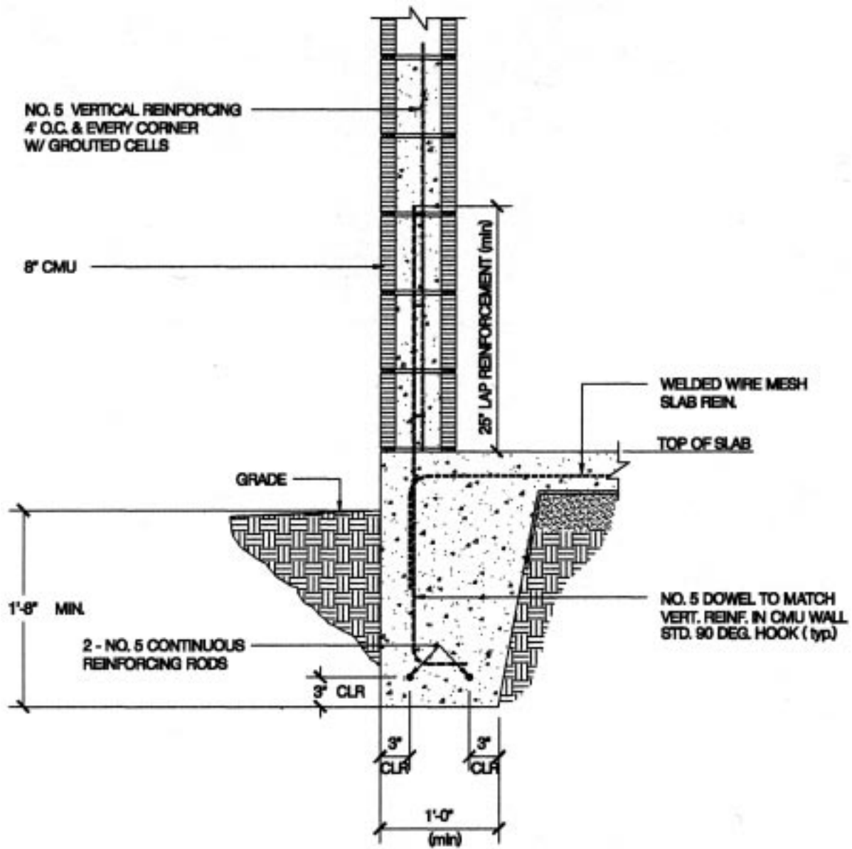
2 SLAB ON GRADE W/ CMU WALL
